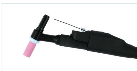
TBi SR 21 (FX) 100% (10 min.) AC: 240 A DC: 340 A Ø 0.5-3.2 mm
